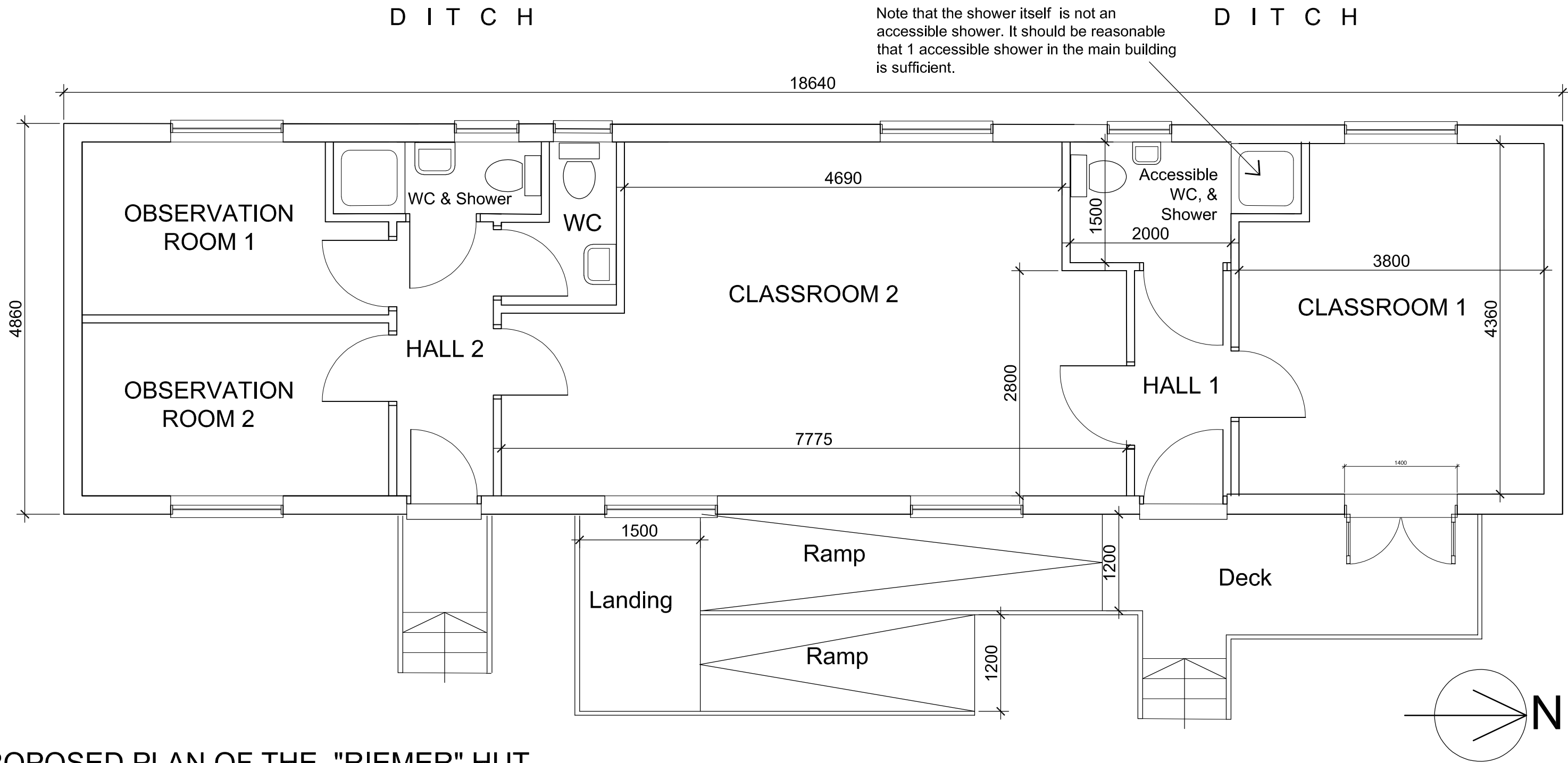
PROPOSED PLAN OF THE "RIEMER" HUT, LOWER FIELD 1:50 at A3 March 2019
